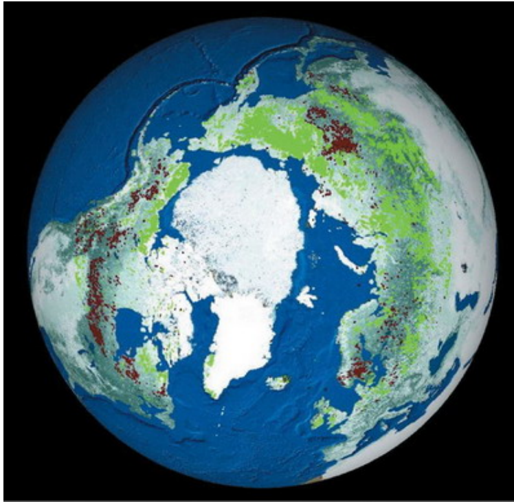
Figure L1. Spatial distribution of trends in May to Aug photosynthetic activity across the northern high latitudes from 1981 through 2005. Significant positive trends in photosynthetic activity are shown in green, and negative trends are shown in rust. (From Bunn et al. 2007.)
