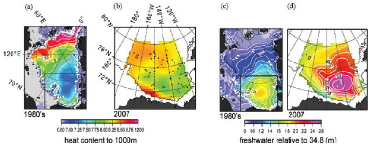
Figure O3. (a), (c) Summer heat ( 1 \times 10^{10} \text{ J m}^{-2} ) and (right) freshwater (m) content in the Arctic Ocean based on 1980s climatology (Timokhov and Tanis 1997). (b), (d) Heat and freshwater content in the Beaufort Gyre in 2007 based on hydrographic survey (black dots depict locations of hydrographic stations). For reference, the Beaufort Gyre region is outlined in black in panels a and c. The heat content is calculated relative to water temperature freezing point in the upper 1,000-m ocean layer. The freshwater content is calculated relative to a reference salinity of 34.8.
