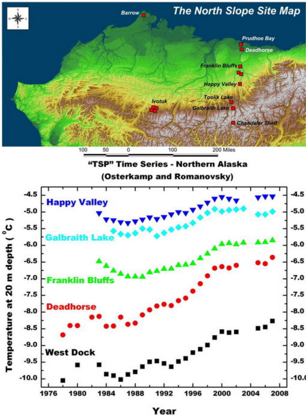
Figure L3. (top) Location of the long-term University of Alaska permafrost observatories in northern Alaska. West Dock is at Prudhoe Bay. (bottom) Changes in permafrost temperatures at 20-m depth during the last 25 to 30 yr (updated from Osterkamp 2003).
