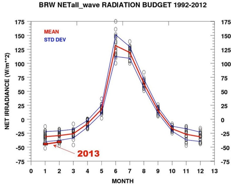
Fig. 9. Mean and standard deviation of net surface radiation (in \text{W m}^{-2} ) at the NOAA Baseline Observatory, Barrow, Alaska, over the period 1992-2012. Net radiation in January and February 2013 is also shown.
