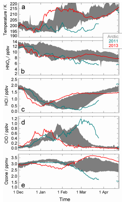
Fig. 13. Averages of high latitude (a) temperatures, (b) nitric acid ( \text{HNO}_3 ), (c) hydrogen chloride ( \text{HCl} ), (d) chlorine monoxide ( \text{ClO} ) and (e) ozone from the NASA Aura Microwave Limb Sounder (MLS) measurements. Measurements made during Arctic winter 2012-2013 (red lines) are compared with those of Arctic winter 2010-2011 (blue-green lines), when unprecedented chemical ozone loss occurred in March 2011 (see the essay on Ozone and UV Radiation in Arctic Report Card 2011). The shaded areas indicate the range of values observed between winter 2004-2005 and winter 2011-2012 (excluding 2010-2011). Concentrations of trace gases are expressed as "mixing ratios" in units of "parts per billion by volume" (ppbv) for \text{HNO}_3 , \text{HCl} , and \text{ClO} , and "parts per million by volume" (ppmv) for ozone. Temperature and mixing ratios refer to the 485 K potential temperature surface (note that the Kelvin [K] unit is always used for potential temperature), at an altitude of \sim 18 km and pressure of \sim 50 hPa, and were averaged over the area of the polar vortex.
