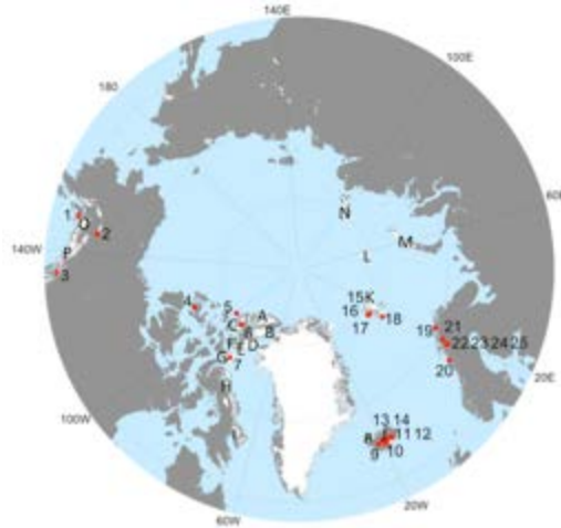
Fig. 50. Locations of Arctic glaciers for which long-term records of climatic mass balance ( B_{\text{clim}} ) are available, and for which recent data are reported here. See Table 6 for glacier names and numbering. Letters represent regions for which MODIS land surface temperature data are presented in Fig. 53 (A: Northern Ellesmere; B: Agassiz; C: Axel Heiberg; D: Prince of Wales; E: Manson; F: Sydkap; G: Devon; H: North Baffin; I: South Baffin; J: Iceland; K: Svalbard; L: Franz Josef Land; M: Novaya Zemlya; N: Severnaya Zemlya; O: South-West Alaska; P: South-East Alaska).
