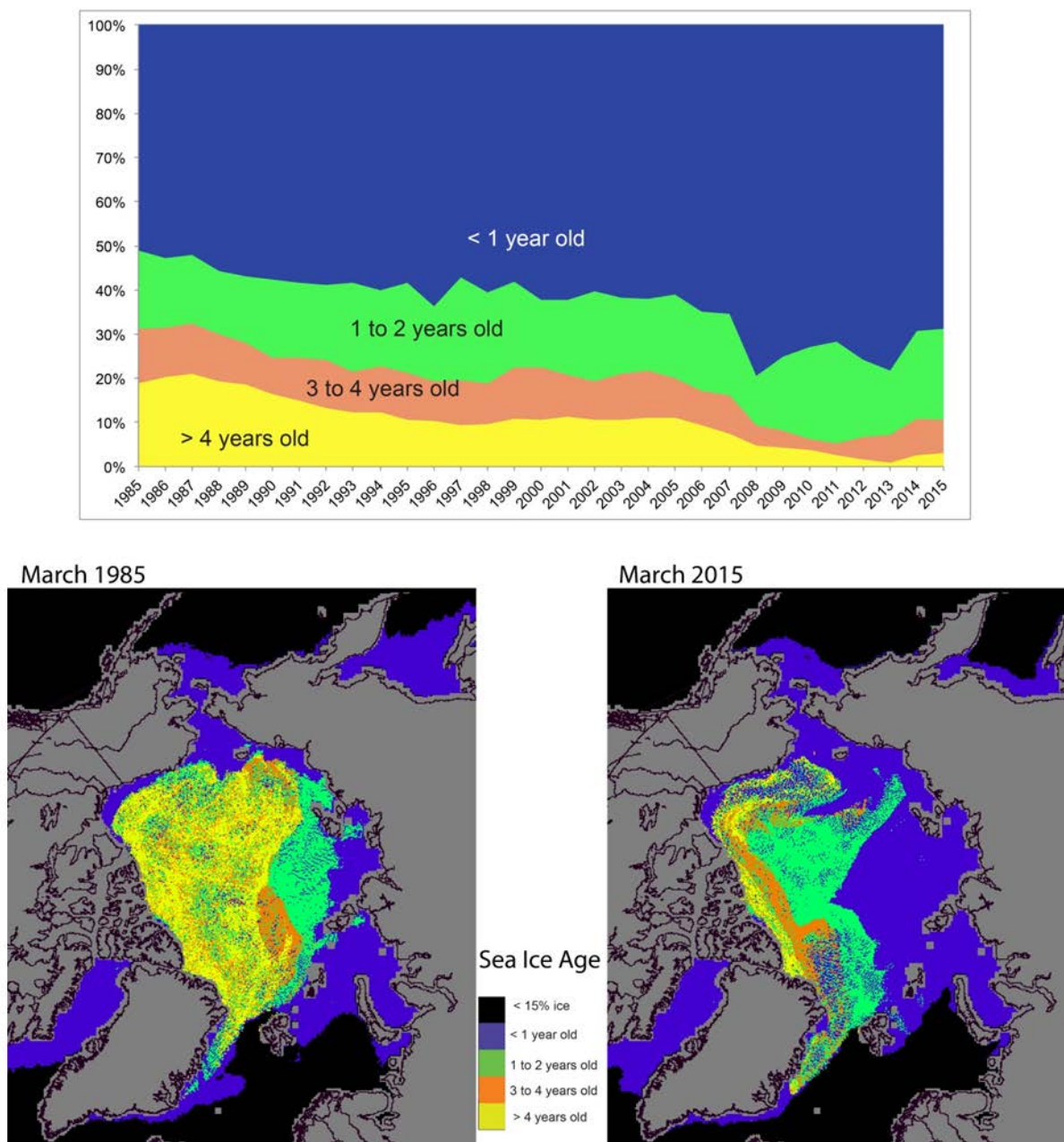
Fig. 4.3. A time series of sea ice age in March from 1985 to the present (a, top) and maps of sea ice age in March 1985 (b, lower left) and March 2015 (c, lower right).
