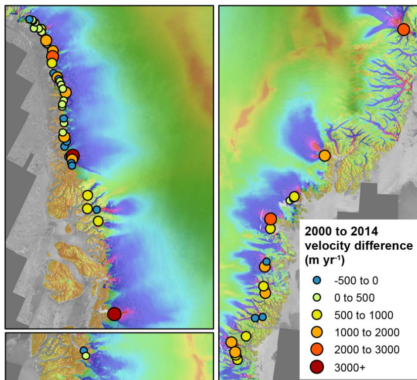
Fig. 12.2. Velocity difference (m yr -1 ) between winter 2000-2001 and winter 2013-2014 measurements for marine-terminating outlet glaciers along the Greenland Ice Sheet western and southeastern coasts. The background image is a composite velocity map derived from InSAR and speckle tracking measurements using the datasets discussed here.
