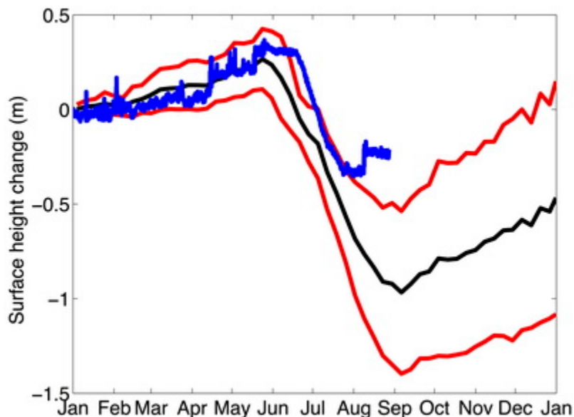
Fig. 3.2. (a, top) The surface mass balance as a function of elevation along the K-transect since balance year 2009-2010. (b, centre) Time series of surface height change at the S5 station at ~540 m a.s.l. on the K-transect. (c, bottom) Same as (b) but for the S9 station at ~1500 m a.s.l. near the equilibrium line on the K-transect. In (b) and (c), the black line is the average for the period 2008-2015 and the red lines indicate 1 standard deviation of the average. Note that in (a), the 91-92 curve is for the period affected by the eruption of Mount Pinatubo, when surface melting was lowered dramatically.
