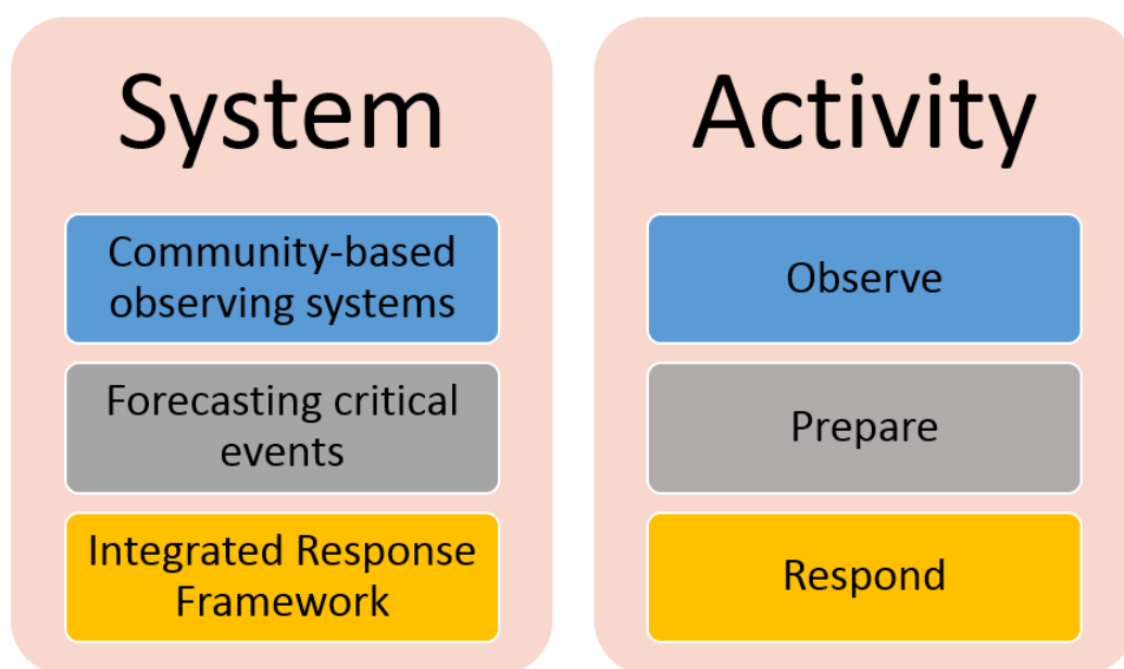
Fig. 11.3. Diagram showing the relationship between observation, preparation, and response activities, in the context of early-warning systems, with corresponding system components for the Arctic: CBONS allow observations to be placed in a situational context; arctic natural and social sciences provide input to the forecasting system, and; an integrated response framework allows targeted preparedness, training and equipment to be mobilized.
