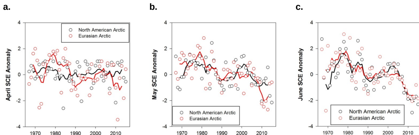
Fig. 2.1. Monthly snow cover extent (SCE) for Arctic land areas ( >60^{\circ}\text{N} ) from the NOAA snow chart CDR for (a, left) April (b, center) May and (c, right) June from 1967 to 2015. Anomalies are relative to the average for 1981–2010 and standardized (each observation differenced from the mean and divided by the standard deviation and thus unitless). Solid black and red lines depict 5-year running means for North America and Eurasia, respectively.
